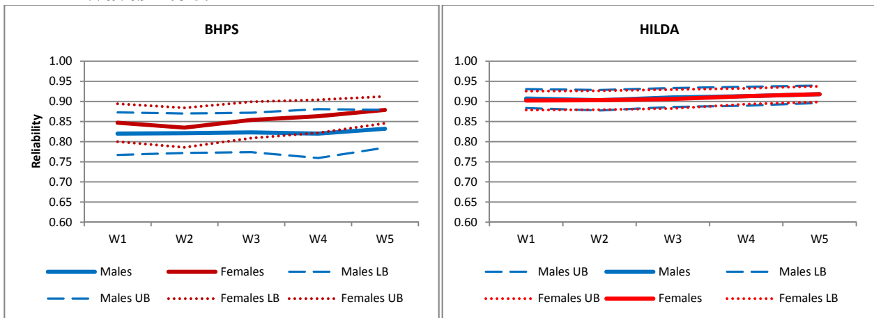
Figure 4 Reliabilities for job tenure from the baseline QSM grouped by sex, BHPS and HILDA Waves 1 to 5.
