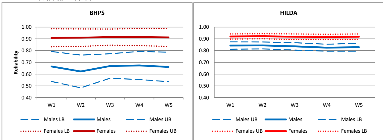
Figure 1 Reliabilities for hours worked from the baseline QSM grouped by sex, BHPS and HILDA Waves 1 to 5.
