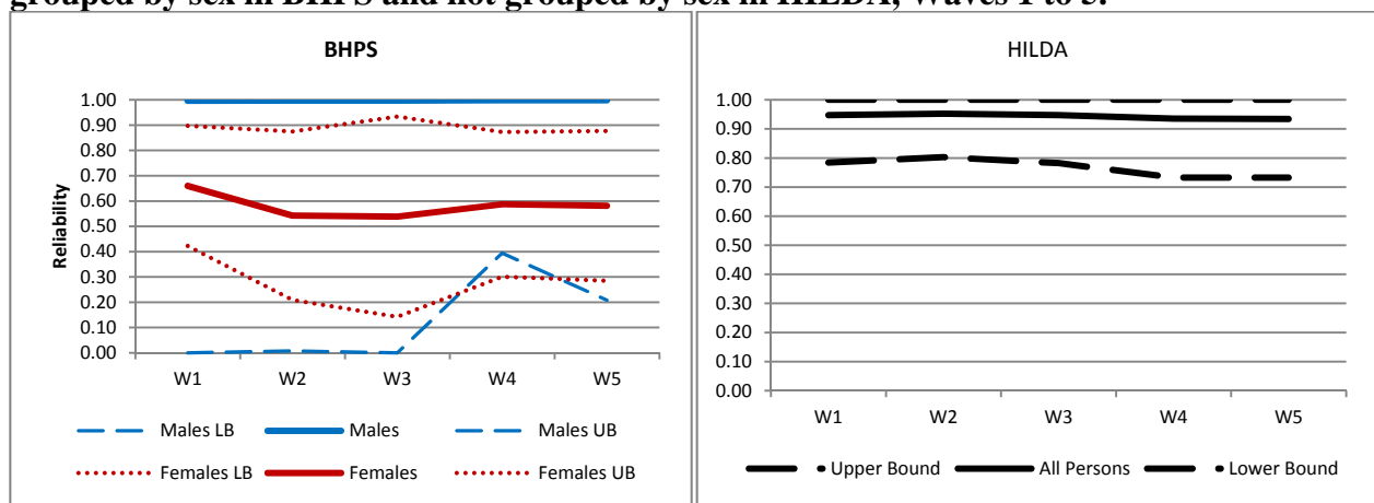
Figure 6 Reliabilities for proportion of the year in employment from the baseline QSM grouped by sex in BHPS and not grouped by sex in HILDA, Waves 1 to 5.
